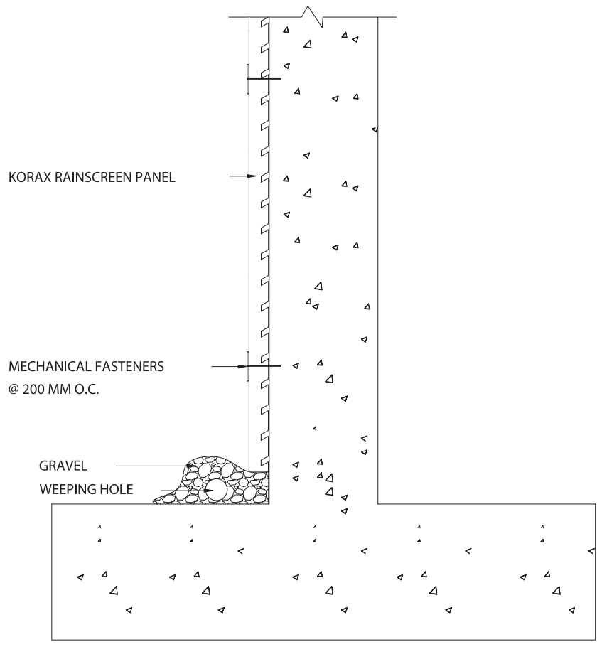
KORAX PANEL USED FOR SUBGRADE DRAINAGE
