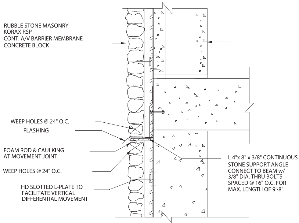
(WITH UNINSULATED CAVITY)
