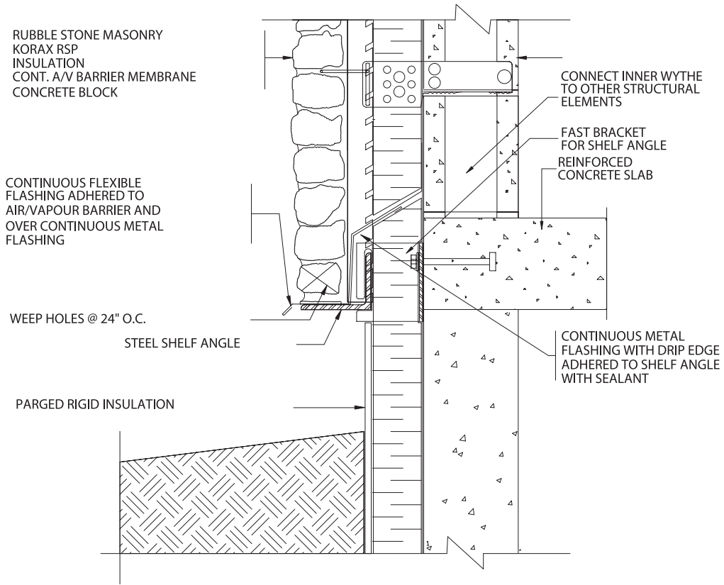
(WITH INSULATED CAVITY)
