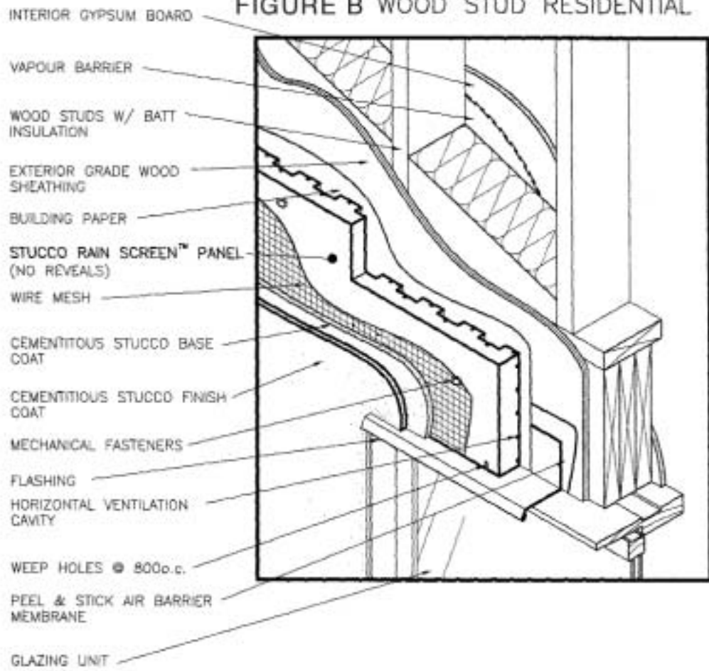
FIGURE B WOOD STUD RESIDENTIAL
