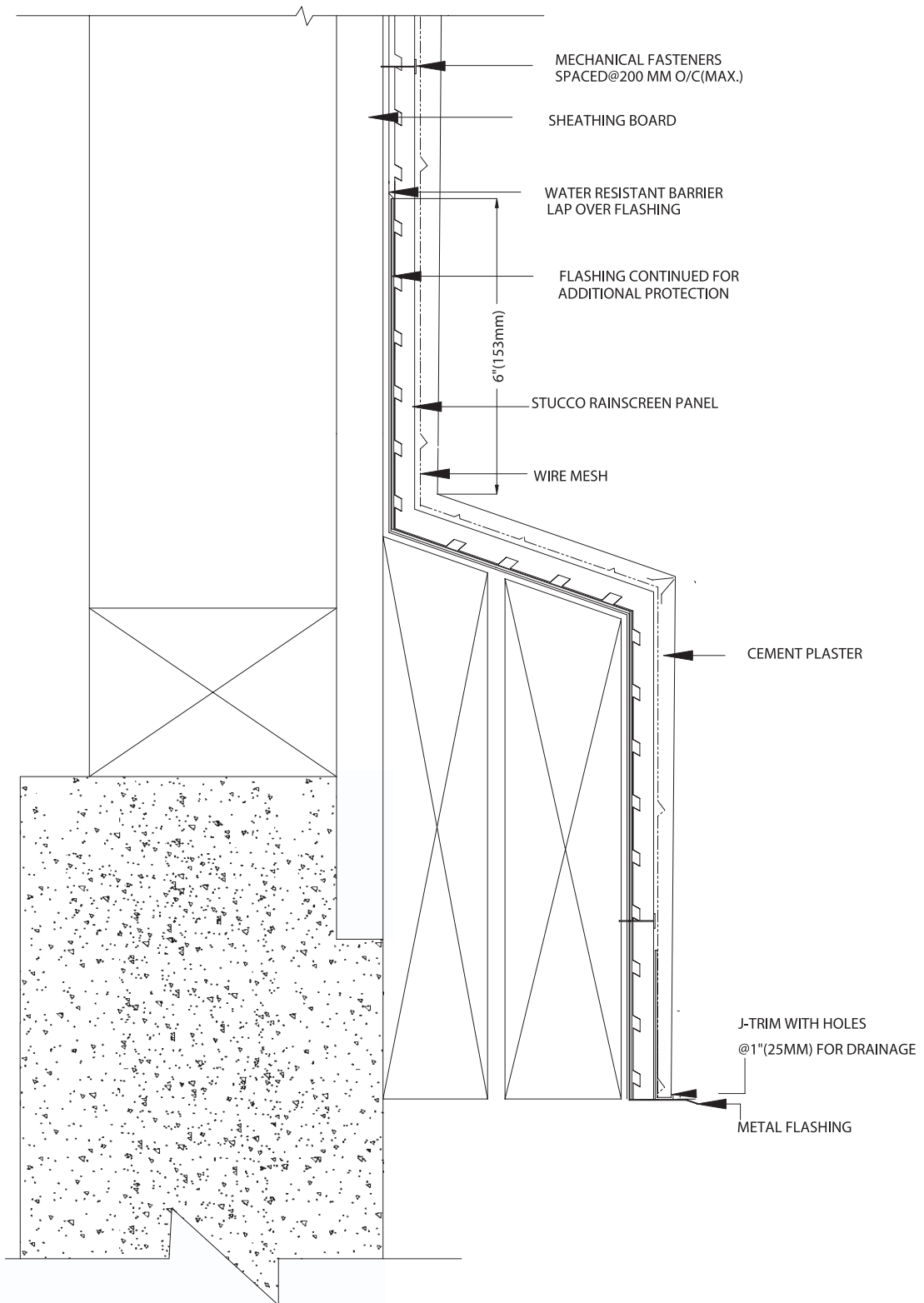
DETAIL 5.7 FOUNDATION/COLUMN TERMINATION
