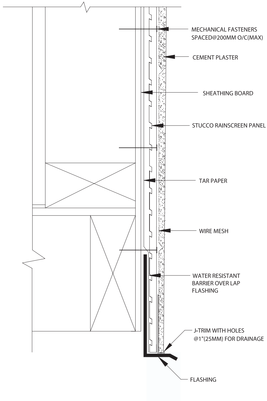
DETAIL 5.5 TERMINATION AT CANTILEVERED WALL
