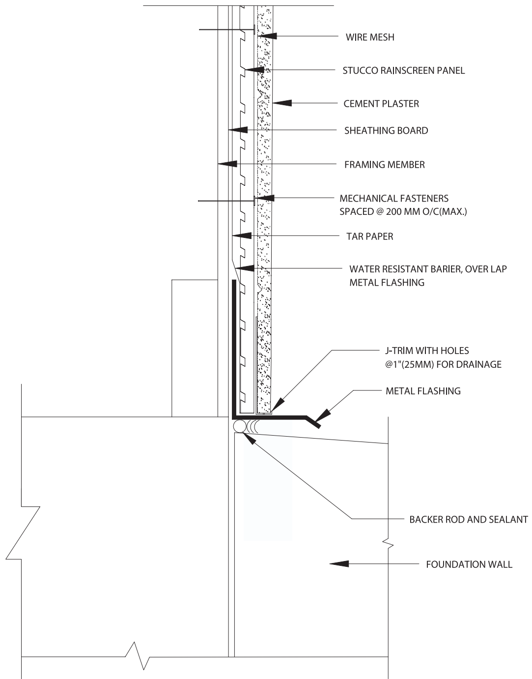
DETAIL 5.4 TERMINATION AT SLAB/SIDEWALK
