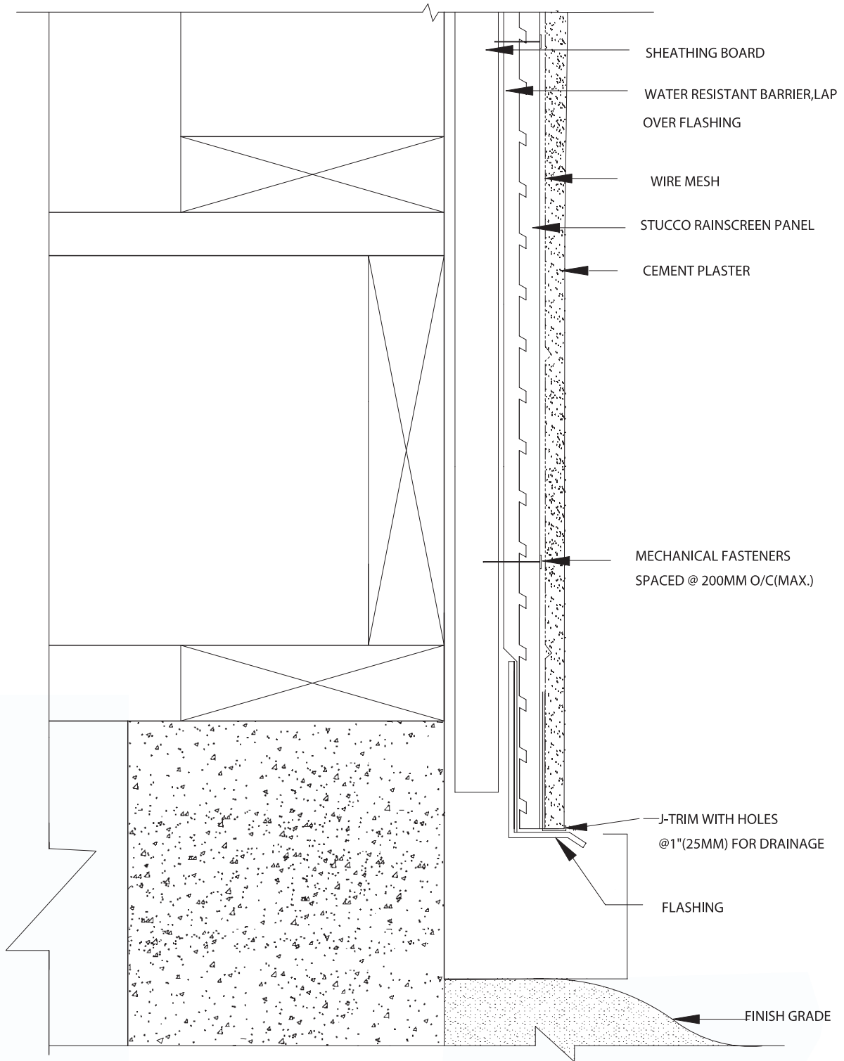
DETAIL 5.3 TERMINATION AT FOUNDATION /FINISHED GRADE
