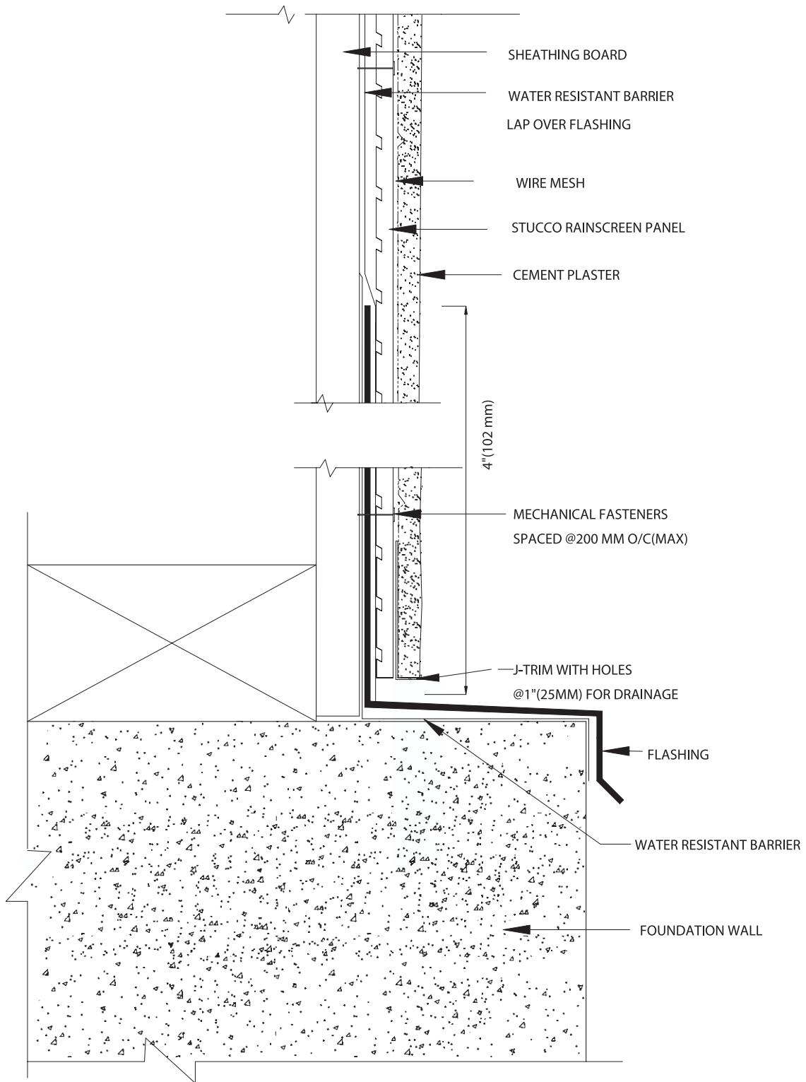
DETAIL 5.1 TERMINATION AT CONCRETE FOUNDATION
