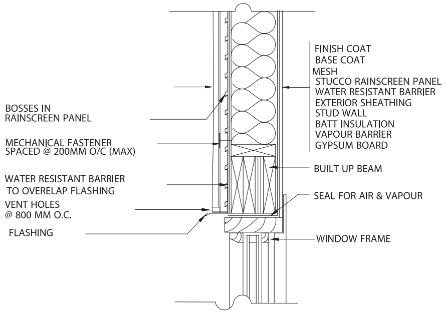
DETAIL 4.4 DETAILS OF WINDOW OPENING WITH CEMENTITIOUS STUCCO
