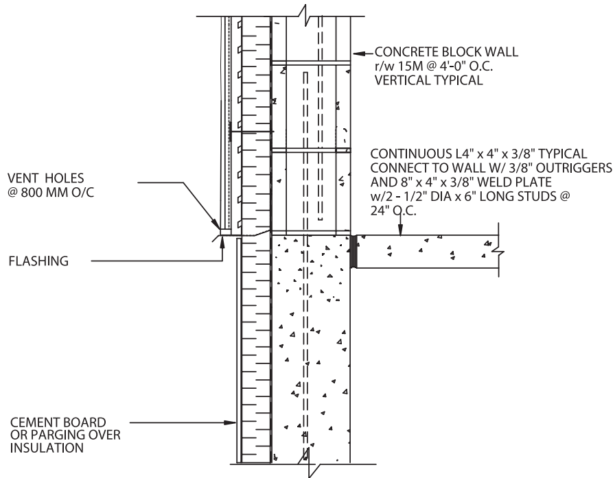
DETAIL 3.7 STUCCO/ CONCRETE BLOCK- AT FOUNDATION
