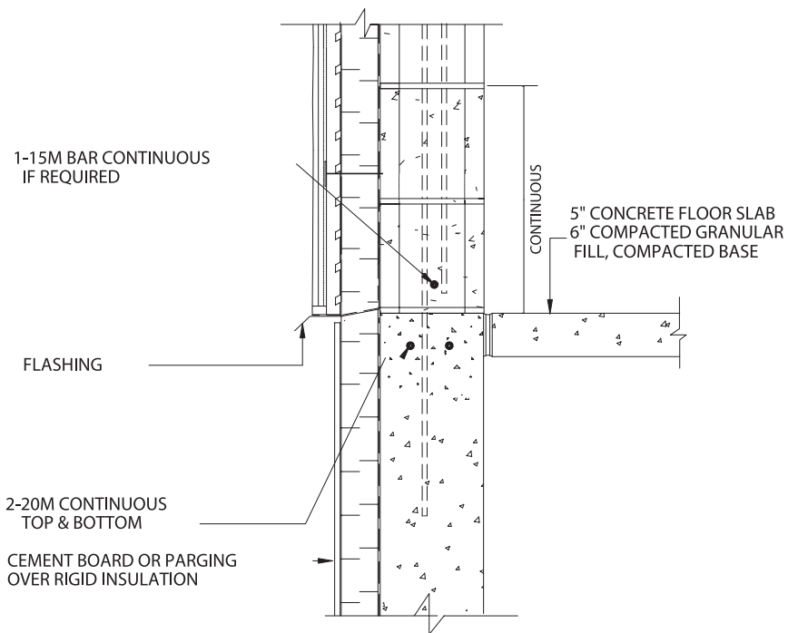
DETAIL 3.6b STUCCO/ CONCRETE BLOCK-AT FOUNDATION BOND BEAM
