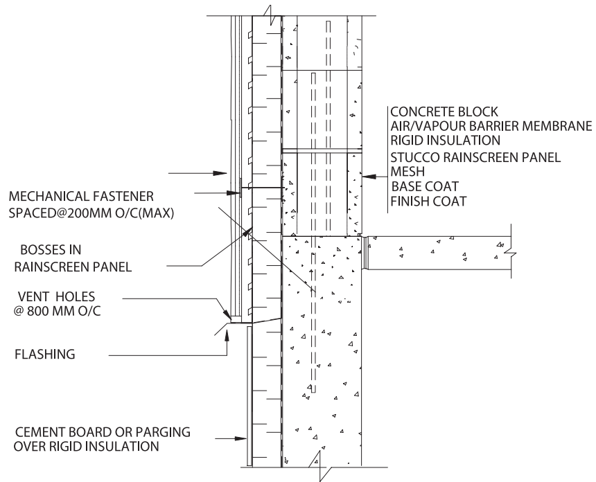
DETAIL 3.6a STUCCO/CONCRETE BLOCK AT FOUNDATION
