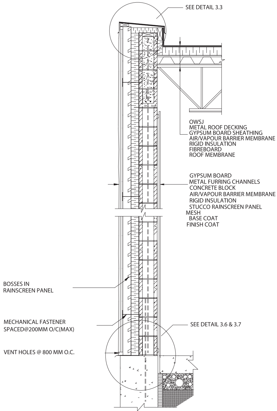
DETAIL 3.2 STUCCO / CONCRETE BLOCK -O.W.S.J. CONNECTION
