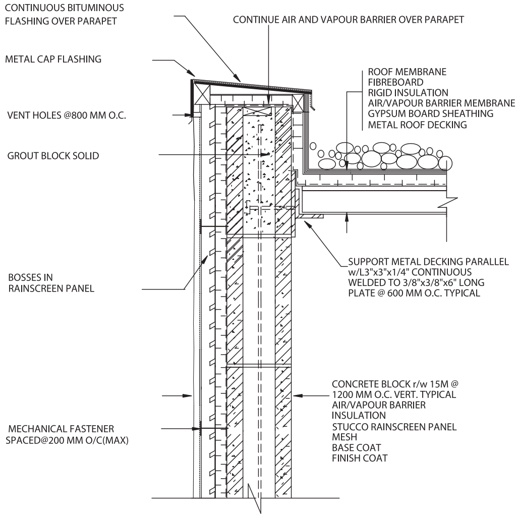
DETAIL 3.1 STUCCO / CONCRETE BLOCK WALL -PARALLEL TO O.W.S.J.
