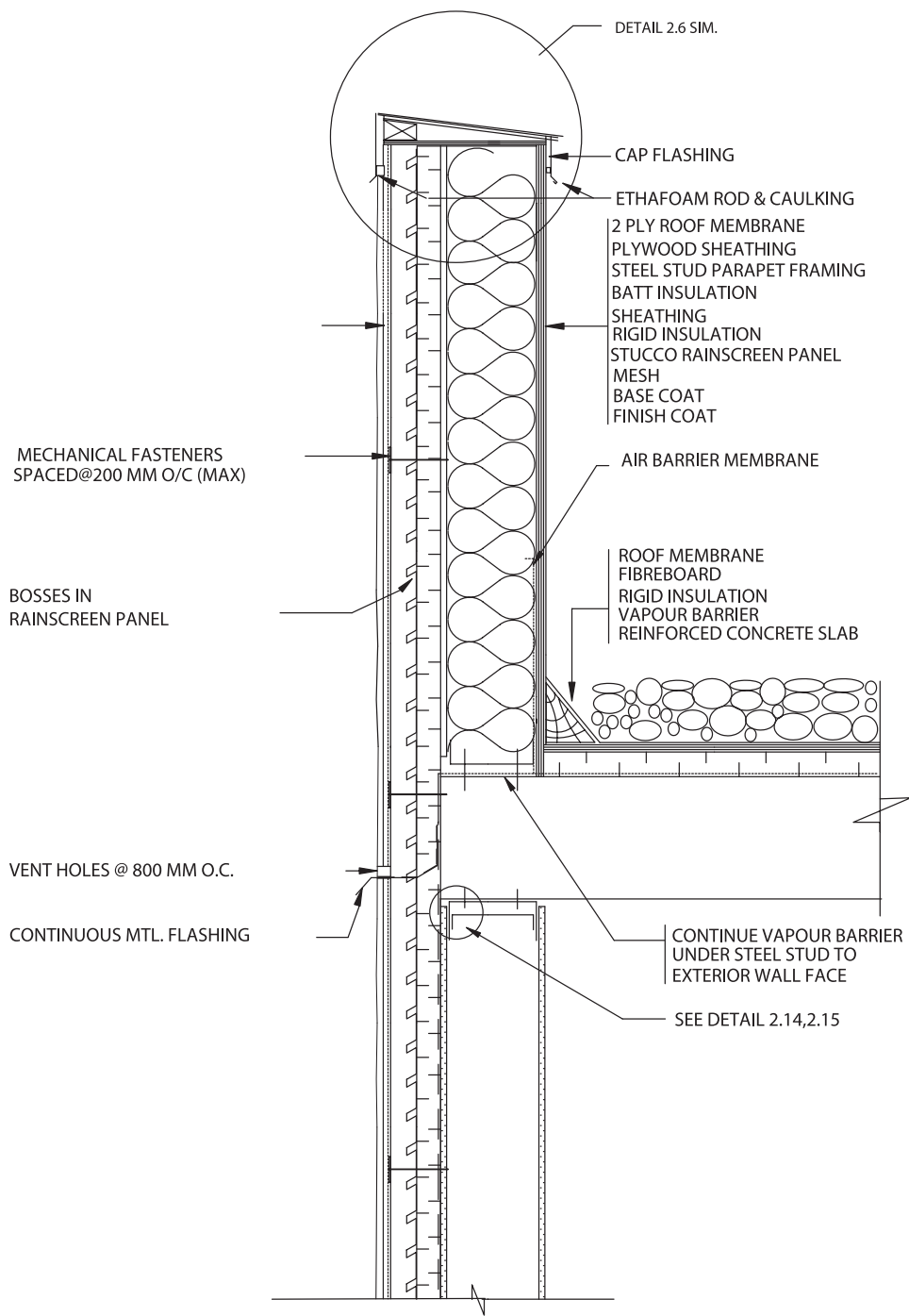
DETAIL 2.7 STUCCO/ STEEL STUD DETAIL AT HIGH PARAPET
