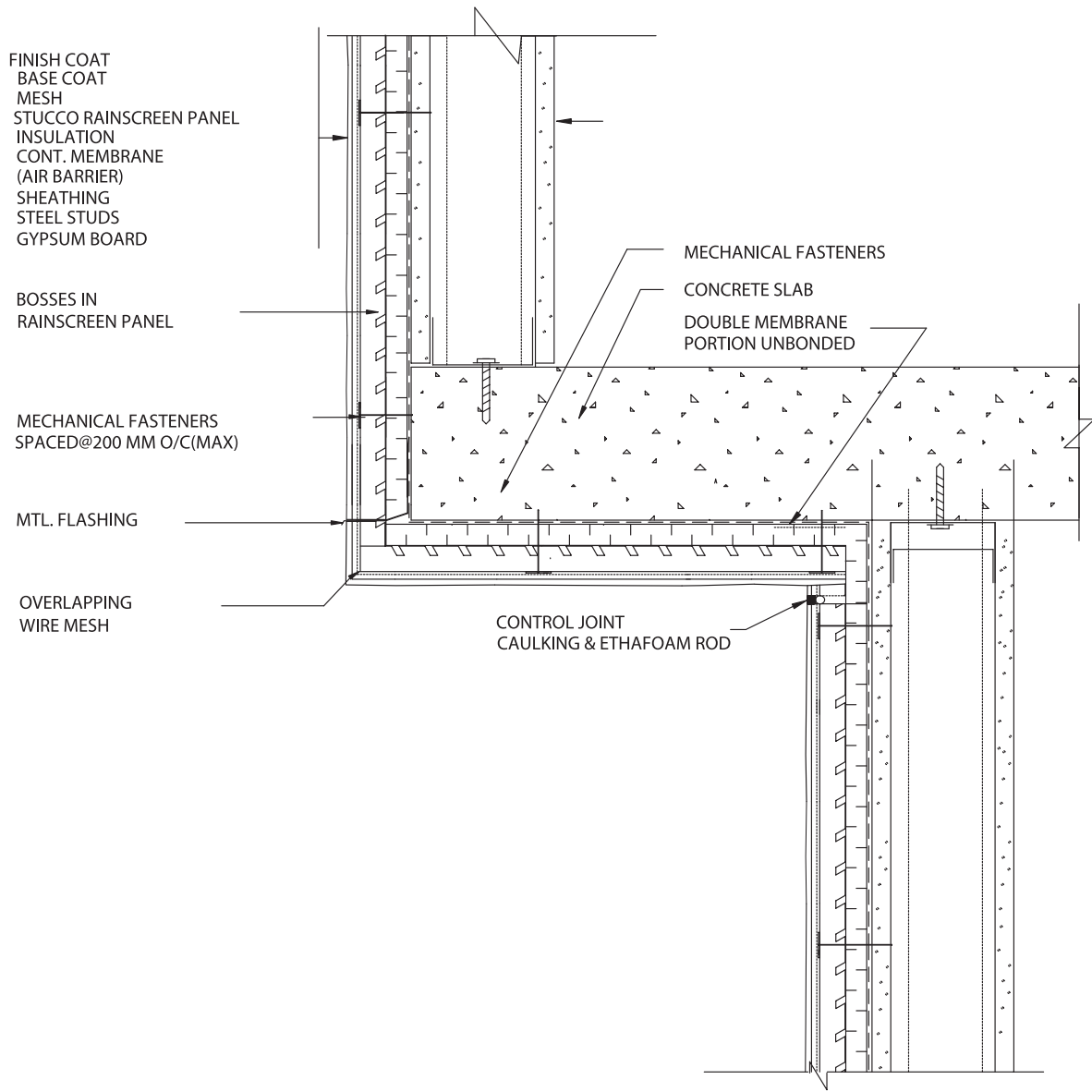
DETAIL 2.11 STUCCO/STEEL STUD-COLD SOFFIT DETAIL
