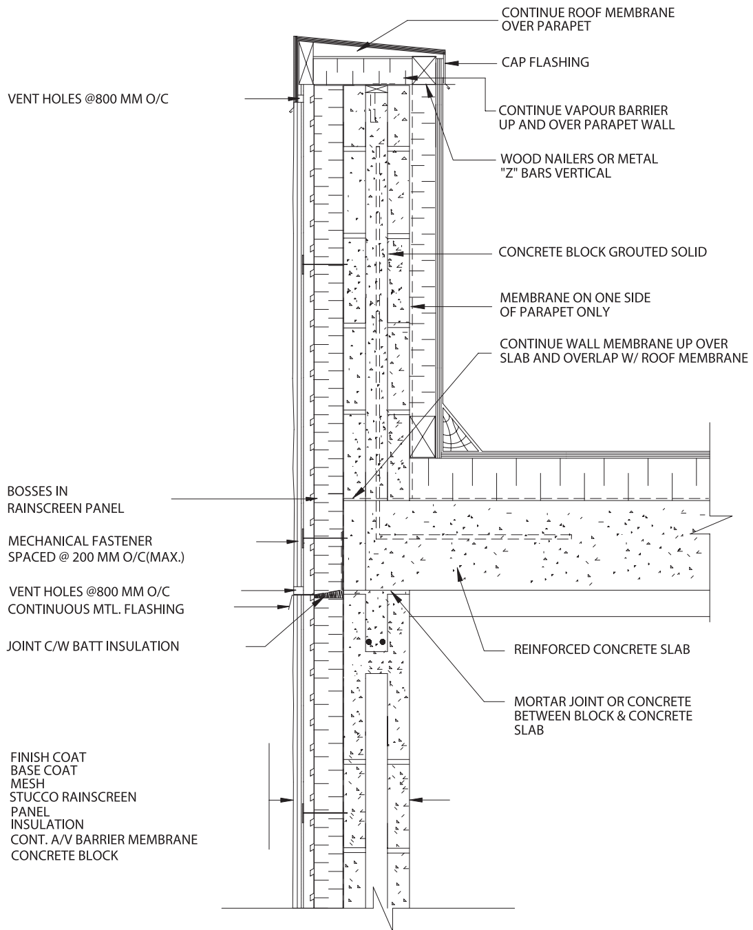
DETAIL 1.8 STUCCO/CONCRETE BLOCK-DETAIL AT HIGH PARAPET FOR LOAD BEARING ASSEMBLY
