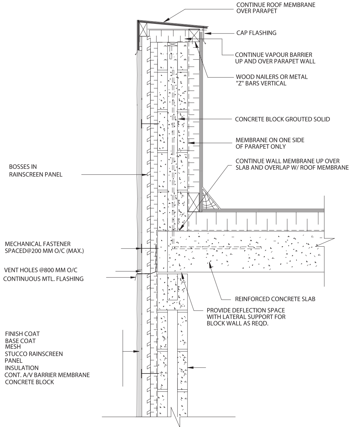
DETAIL 1.7 STUCCO/CONCRETE BLOCK-DETAIL AT HIGH PARAPET FOR NON LOAD BEARING ASSEMBLY
